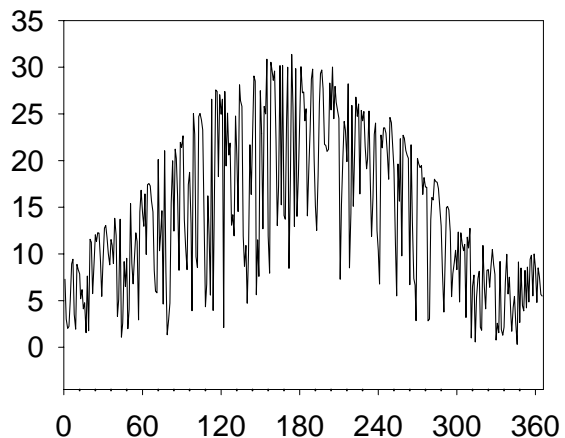
Shortwave Radiation (MJ m -2 d -1 )
